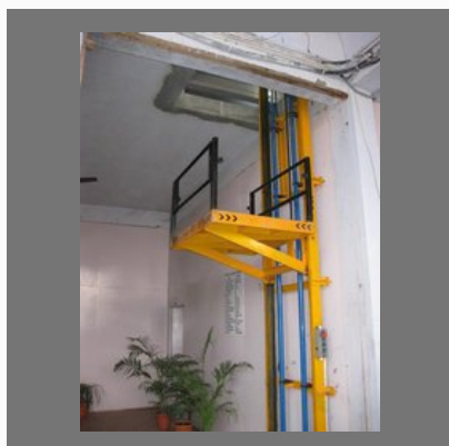
Hydraulic Wall Mounted Goods Lifts
